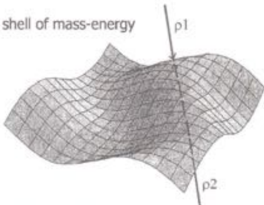
Figure 5. A Thin Shell of (Localized) Mass-Energy Possessing Two Principal Radii of Curvature, \rho_1 and \rho_2 .
