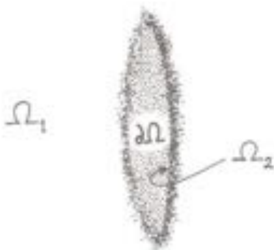
Figure 4. The Same Diagram as in Figure 3 Except as Viewed by an Observer Sitting in Region \Omega_1 , Who Looks Through the Wormhole Throat \partial\Omega and Sees Remote Region \Omega_2 , (dotted area inside the circle) on the Other Side
