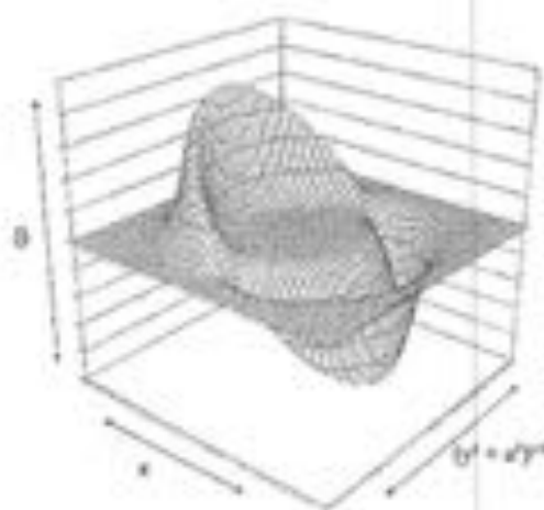
Figure 1. York Extrinsic Time ( \beta ) Plot
